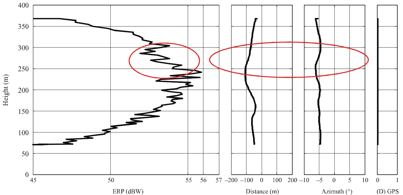
Vertical diagram with flight information
