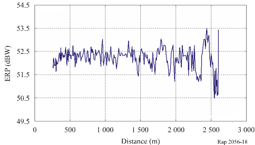
Propagation diagram 5 dB range
